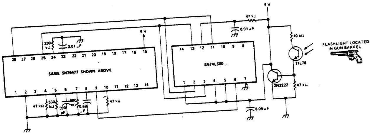
ADDITIONAL CIRCUITRY FOR SILENCER AND GUN SHOT (FOR USE WITH BIRD SOUNDS ABOVE)
